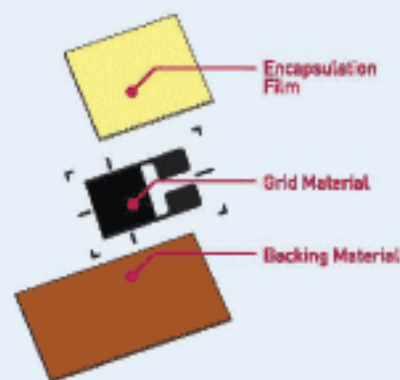
Strain Gauge Structure
